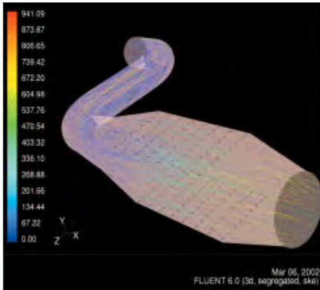
Figure 4. Model Output Showing Particles Tracked Trough UV Unit to Calculate Applied UV Dose.
